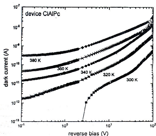
Fig. 1: Temperature variatioll of the I-V characteristic in reverse bias for CIAIPc.
