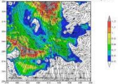
EMISSION FRICTION(m/s) & STREAMLINES 09Z15July2011
