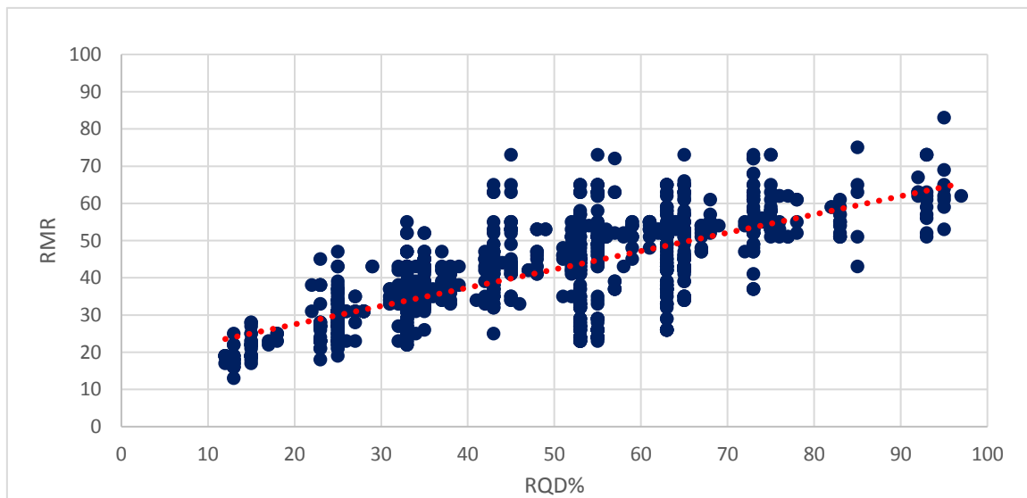
Fig. 4. The relationship between RMR value and Rock Quality Designation (RQD) index
