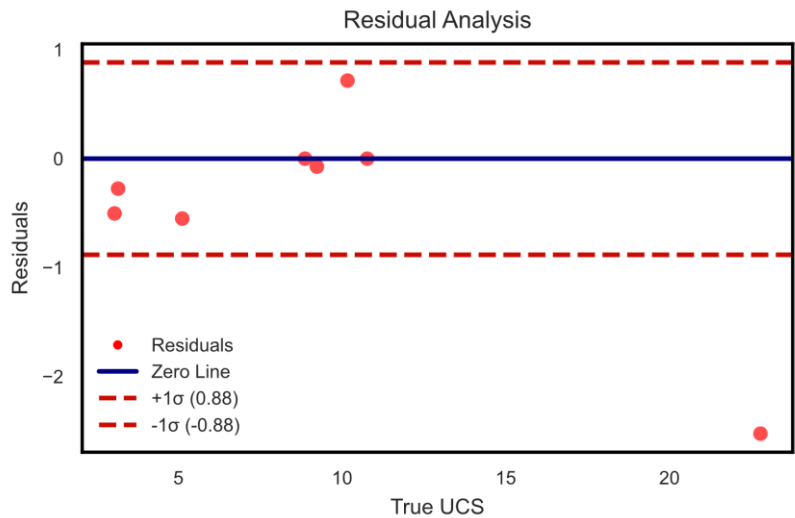
Fig. 9. Residual analysis to identify systematic biases
