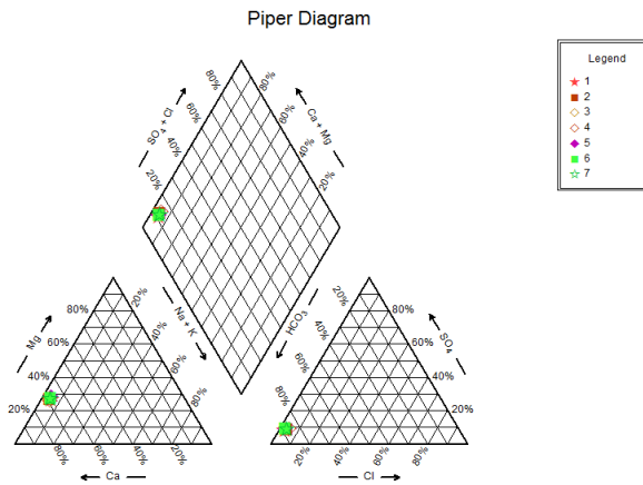
Fig. 3. Piper diagram of Vorskaharan spring water samples
