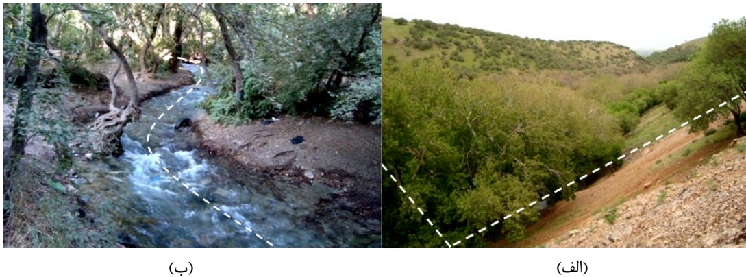
Fig. 5. An image of a) the valley shape and b) the meanders of the Gian River
