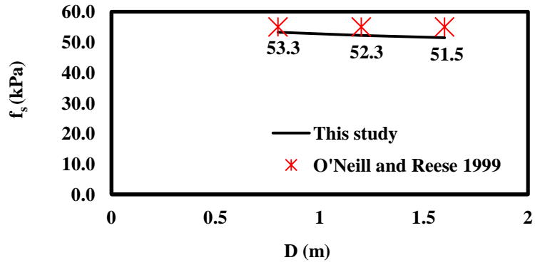
Figure 15. Effect of pile diameter on side resistance
