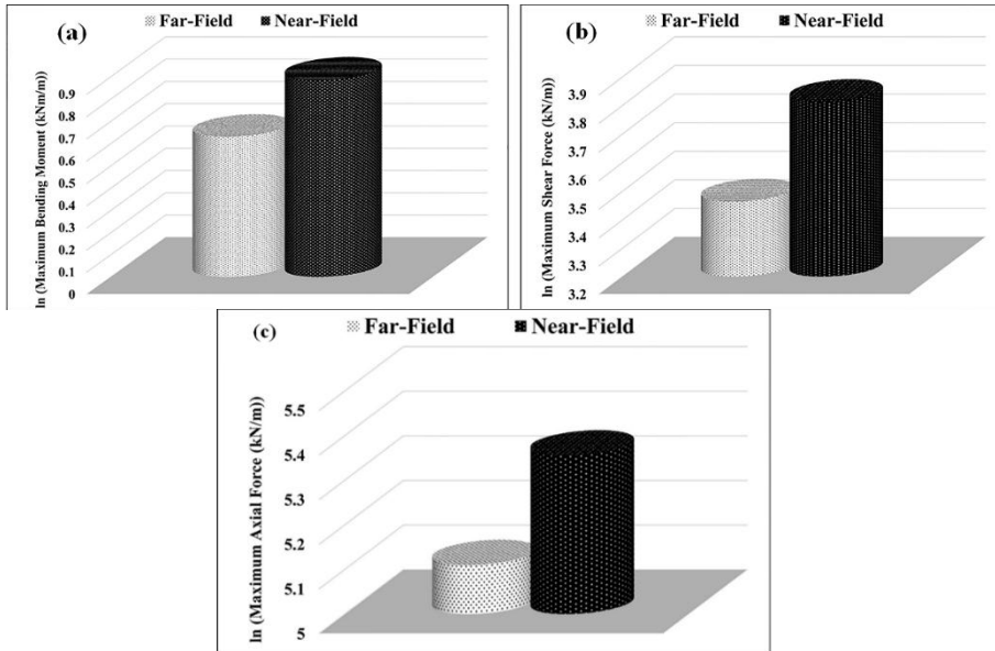
Figure 9. Comparison of the logarithmic averages of (a) bending moment, (b) shear force and (c) axial force in the nails under the effect of near-fault and far-fault ground motions
