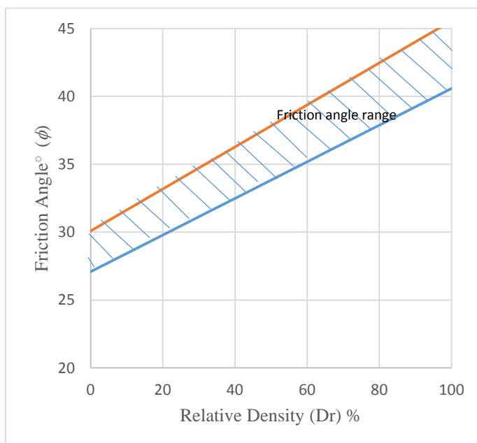
Figure 1. Internal friction angle range of silicate sands for different relative densities (Baziar and Salehzadeh [9])
