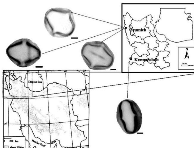
Fig. 2. Distribution and pollen photomicrographs of 4 taxa of A. sect. Macrophyllum in Iran. Scale bar = 6 µm.
