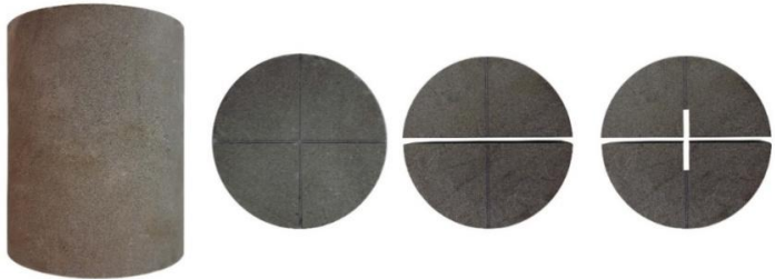
Figure 6. Preparation of the SCB specimen
