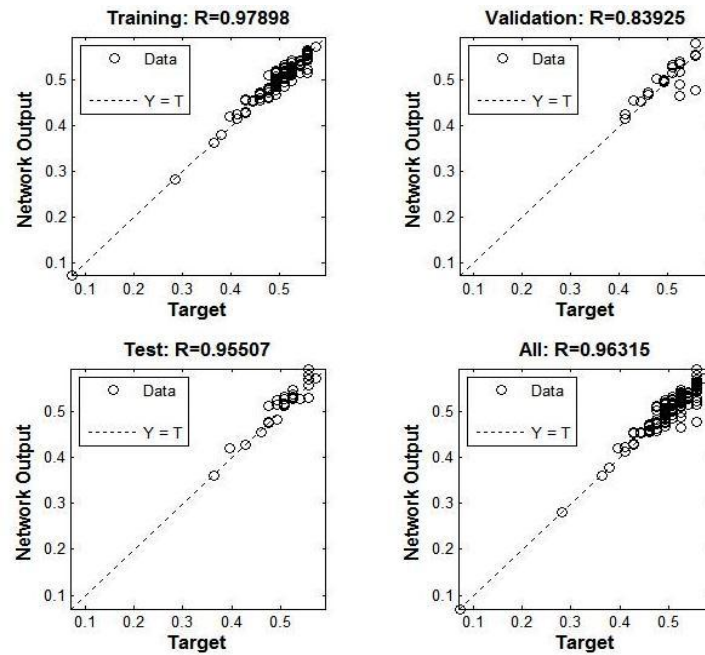
Figure 7. Correlation factor between measured and predicted surface Settlement
