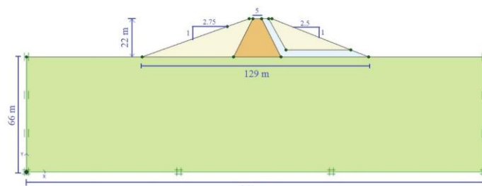
Figure 3. Model geometry
