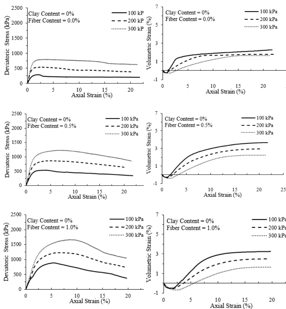
Figure 2. Deviatoric stress-axial strain (on the left) and volumetric strain-axial strain curves (on the right) of unreinforced and fiber-reinforced samples with D_r = 50\% and clay content = 0%
