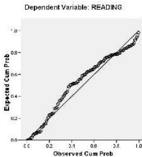
Figure 2: Regression model for the measures
